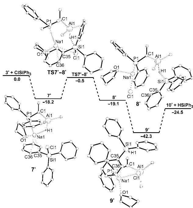
Figure 2. Relative M06-2X/6-31G(d) energies (zero-point energy corrected, in kcal mol −1 ) for the conversion of 3' and ClSiPh 3 into 10' and HSiPh 3 via reactant complex 7' and product complexes 8' and 9' . Hydrogen atoms (except H1) are omitted for clarity. Selected average bond lengths [pm] and angles [°] for 7' : Al1–H1 167.0, H1–Na1 212.9, Na1–P1 303.4, Na1–C35 285.3, Na1–C36 284.1, Si1–Cl1 210.9. TS7'-8' : Al1–H1 180.0, H1–Si1 175.6, Si1–Cl1 228.4, Na1–P1 299.3, Na1–Cl1 293.0, Na1–C35 266.7, Na1–C36 274.9; H1–Si1–Cl1 77.6. 8' : Al1–H1 194.4, H1–Si1 152.3, Na1–P1 184.8, Na1–Cl1 247.7. 9' : Al1–Cl1 231.2, Cl1–Na1 262.2, Na1–P1 285.8, Na1–C35 285.6, Na1–C36 284.7, Si1–H1 148.3.
